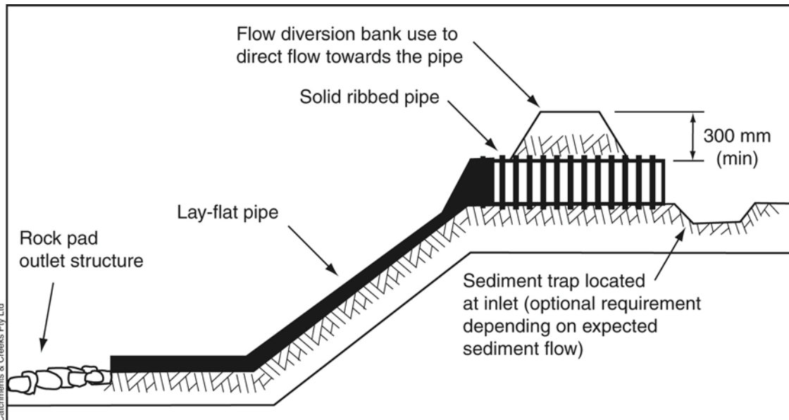
Figure 2 – Slope drain formed from lay-flat pipe
