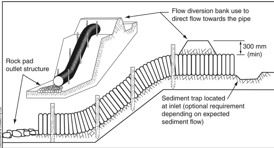
Figure 1 – Slope drain formed from flexible PVC pipe
