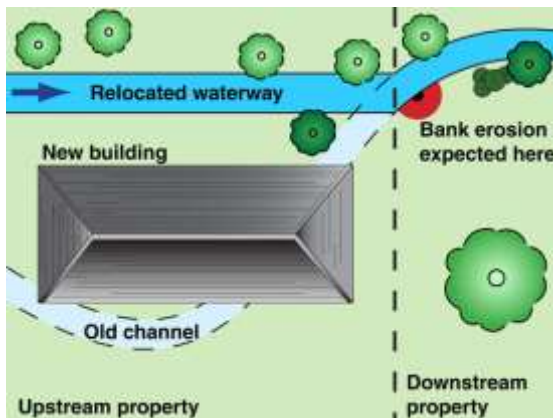
Relocated waterway channel
