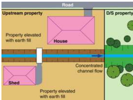
Concentration of channel flow
