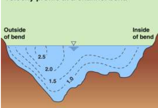
Velocity profile at a channel bend
