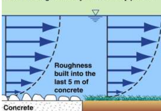
Roughness added to concrete surfaces
