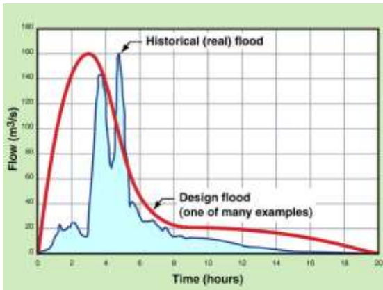
Example historical and design floods
