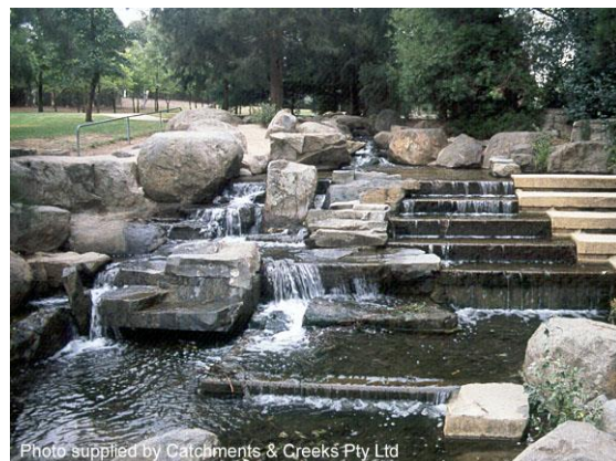
Grouted rock stepped spillway (ACT)
