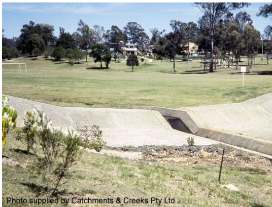
Trapezoidal, inclined drop structure (Qld)
