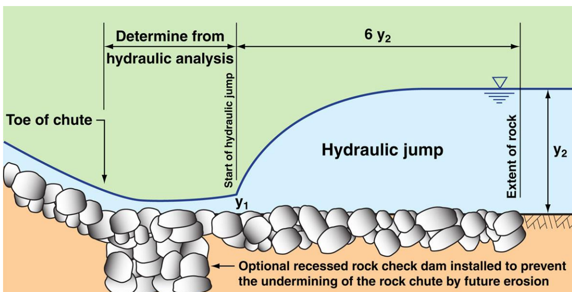
Rock chute with bed-level crest and no pools
