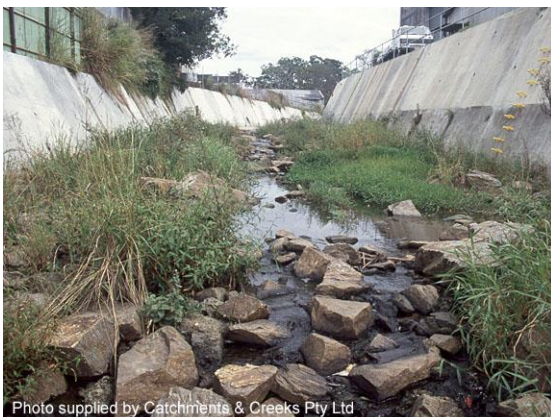
Rocks grouted to concrete channel (Qld)
