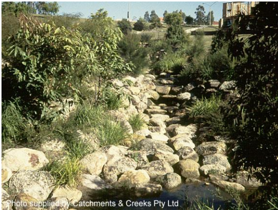
Grouted rock chute (Qld)
