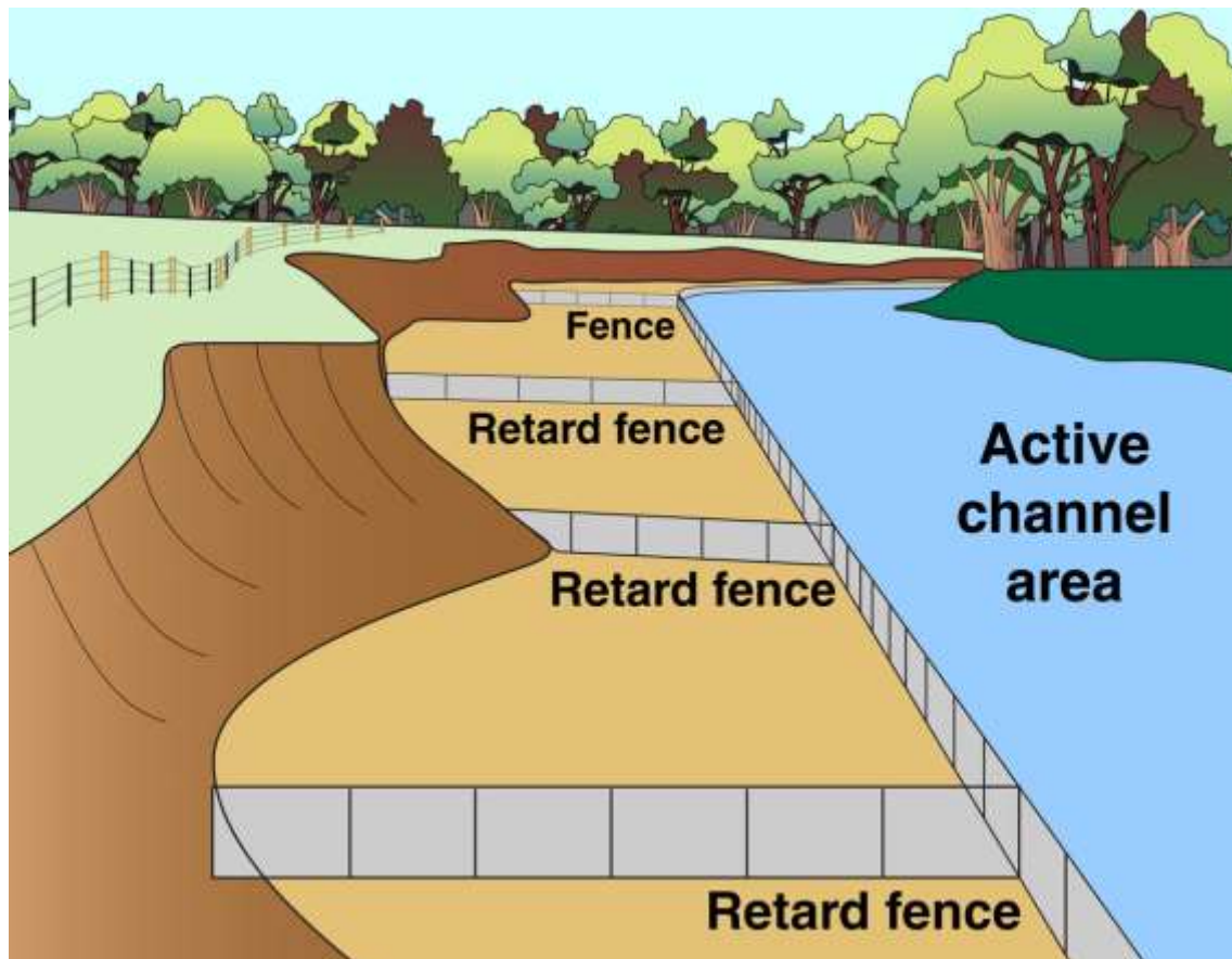
Retard fencing
