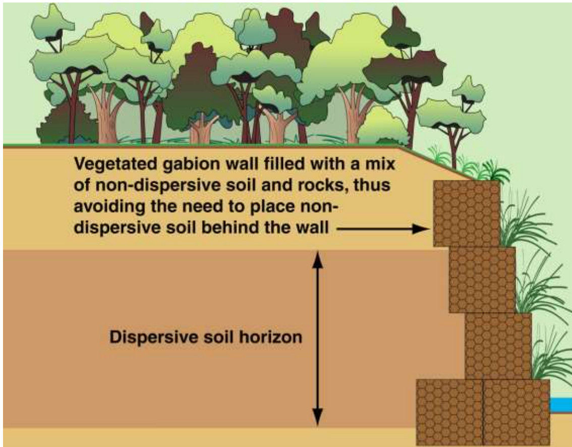
Non-dispersive soil in the vegetated gabion wall helps to retain the disperse soil
