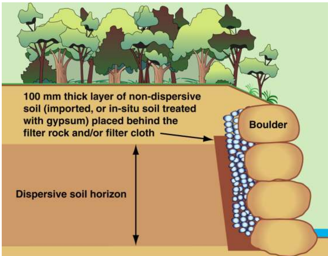
Stacked boulder wall adjacent a disperse soil horizon
