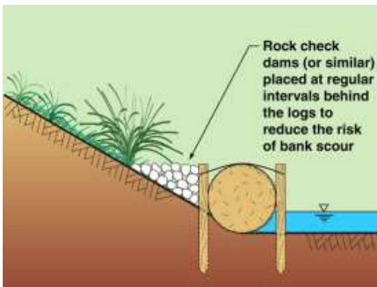
Use of rock check dams to control scour
