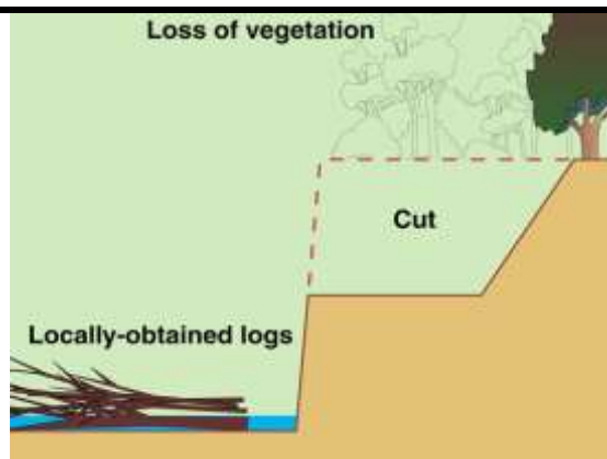
Stage 1: Cut bank and place felled trees
