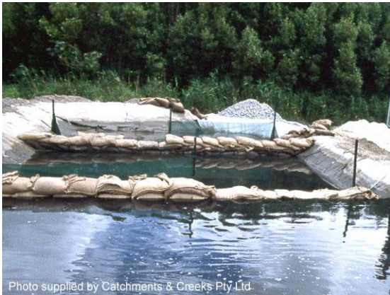
Outflow from the settling pond
