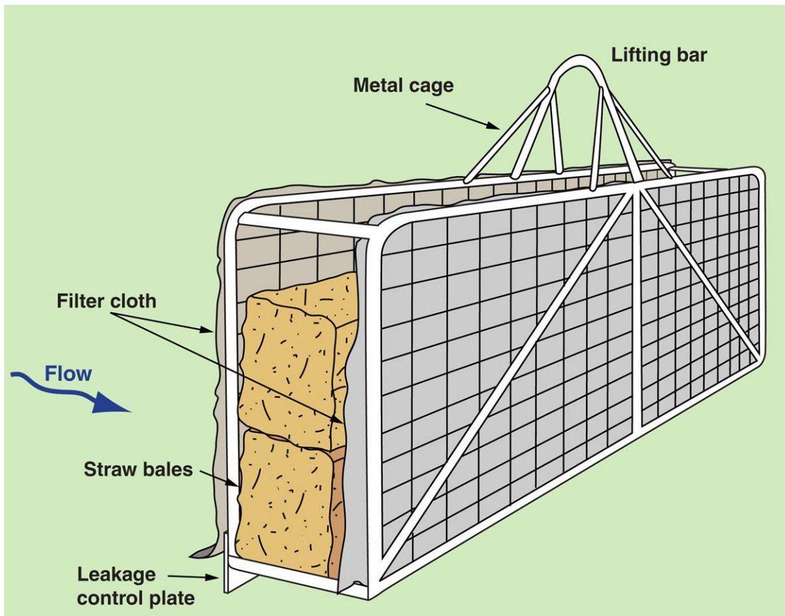
Filter cage
