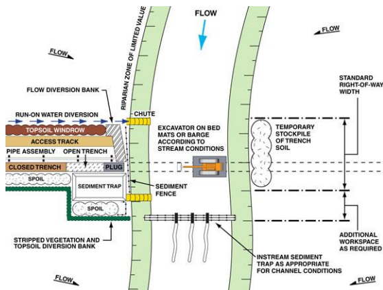
Shallow-bed waterway
