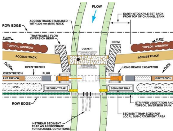
Minor waterway
