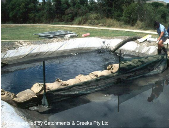
Stage 1 of settling pond (inlet)
