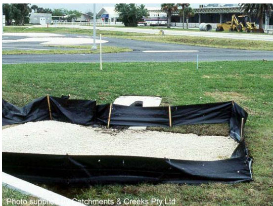
Gravel soakage (infiltration) pit (USA)
