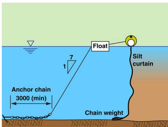
Marine anchor
