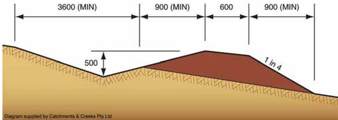
Narrow width cross drainage berm (for low speed tracks)
