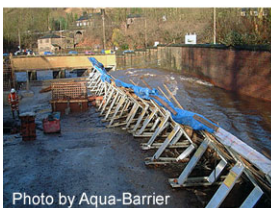
A-frame Aqua Barrier
