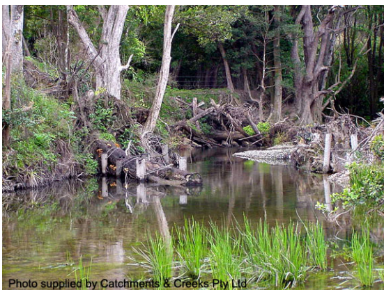
Log groynes
