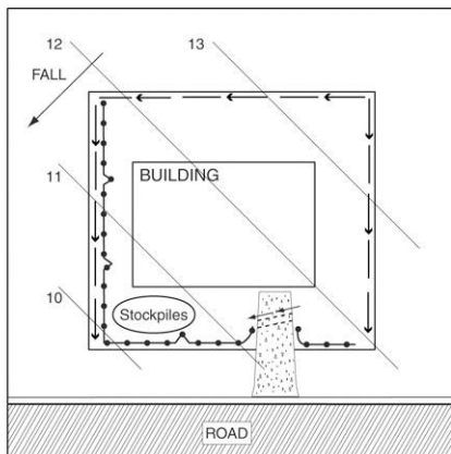
Stockpile located away from overland flow
