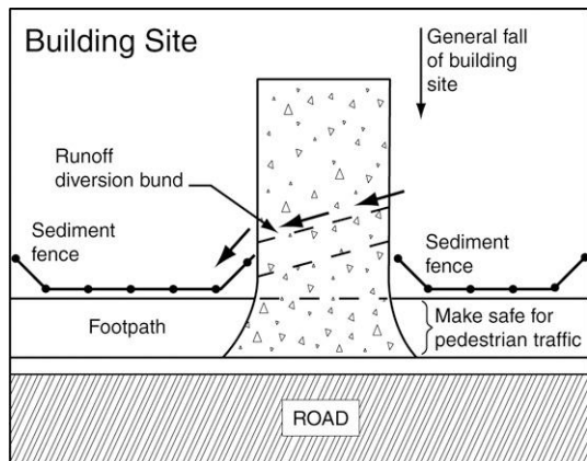
Rock entry/exit pad
