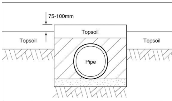
Backfilling of a service trench
