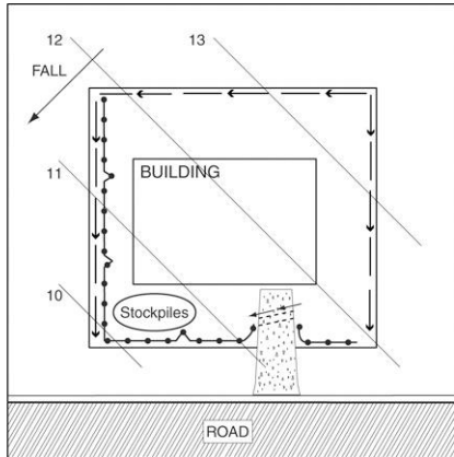
Erosion & Sediment Control Plan
