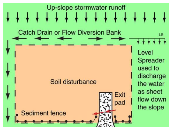
Diversion of driveway run-off
