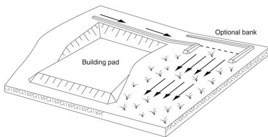
Use of a level spreader to release flows
