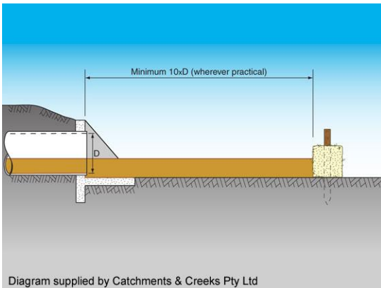
Example of above-ground ponding
