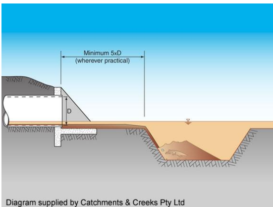
Excavated sediment trap at pipe outlet
