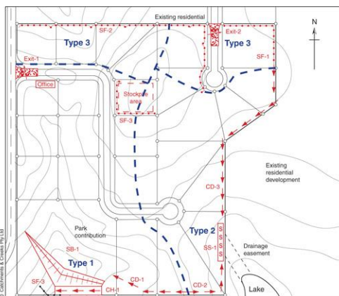
Site controls based on erosion risk
