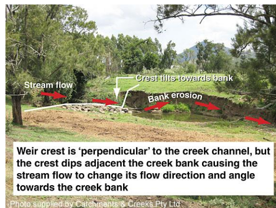
Bank erosion produced from weir (left)
