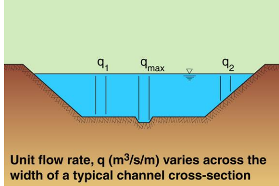
Defining the unit flow rate (q)
