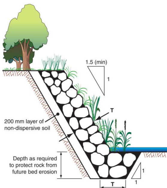
Diagram supplied by Catchments & Creeks Pty Ltd Vegetated rock placement over poor soils
