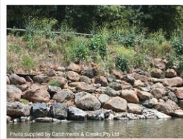
Photo 1 – Lower bank rock stabilisation with voids filled with small rocks
