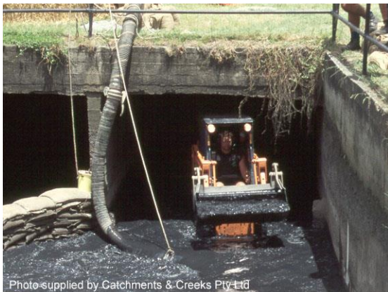
De-silting operation (Qld)
