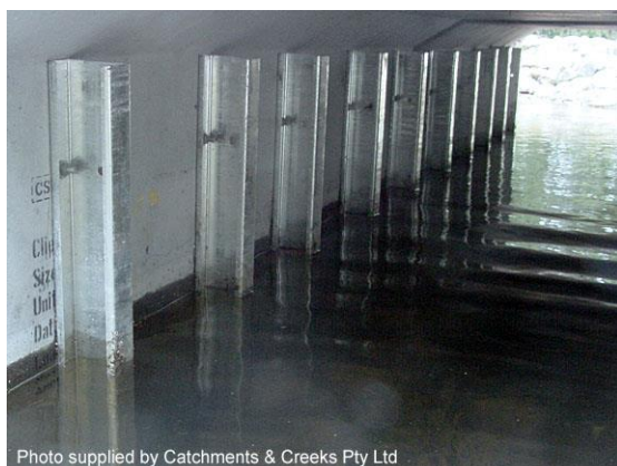
Sidewall baffles (NSW)
