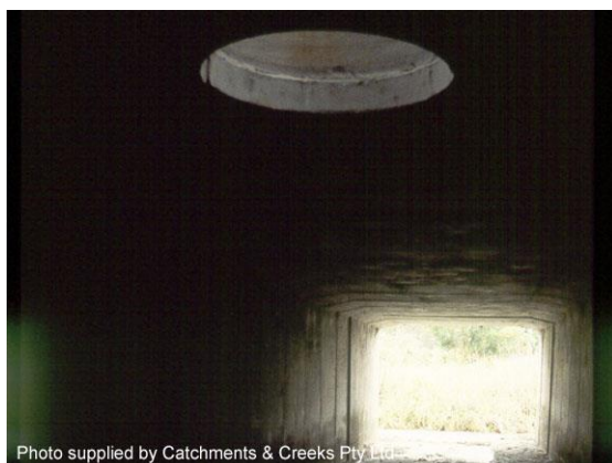
Skylight in the roof of a box culvert (Qld)
