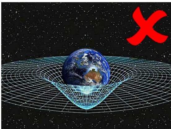
Curved spacetime
