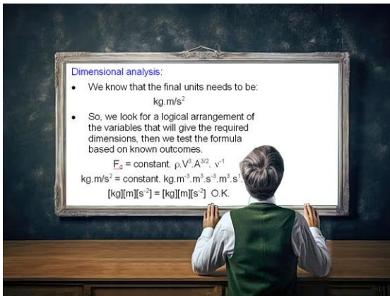
Dimensional analysis
