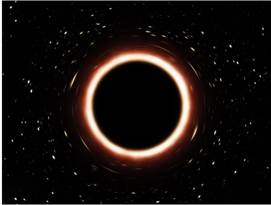
Black hole
