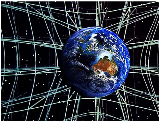
Spacetime
