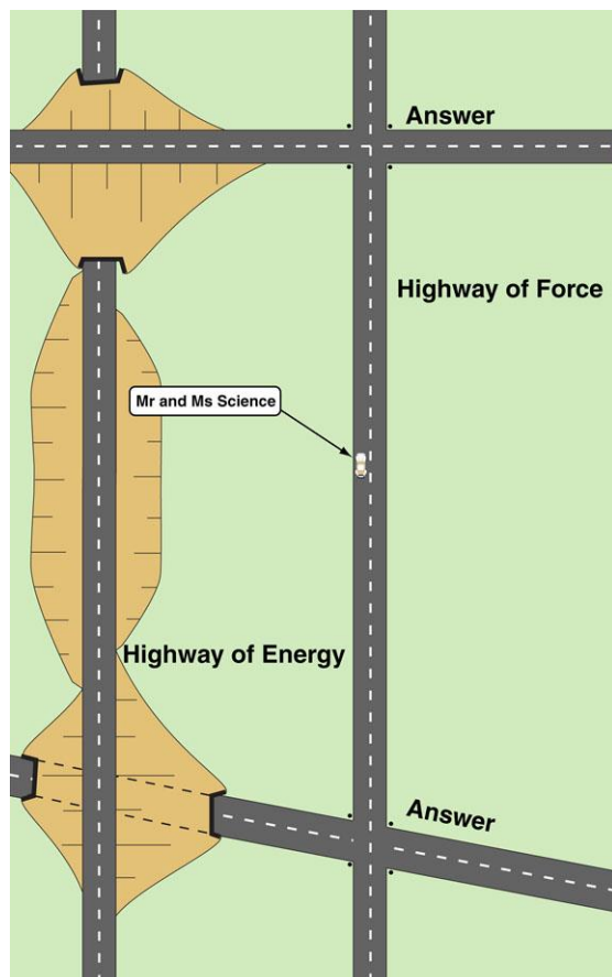
Force-based model
