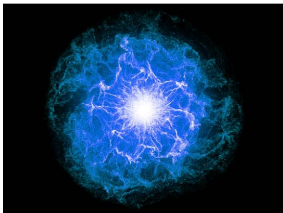
Early expansion
