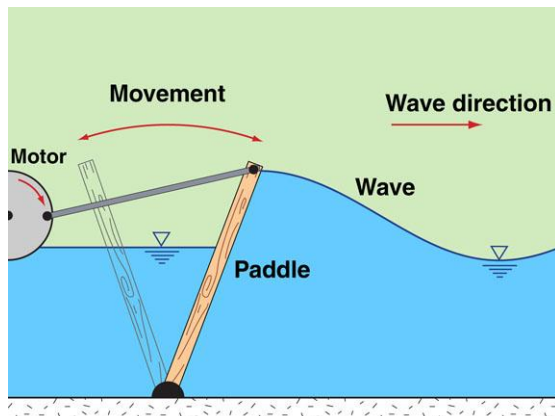
Wave paddle
