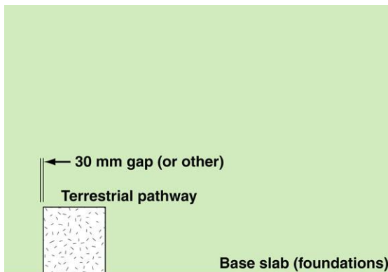
Foundations
