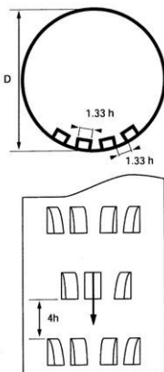
Ridge-block fishway (Walaman)
