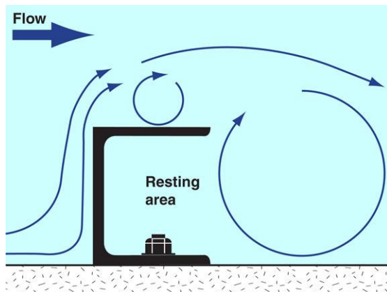
Channel baffle
