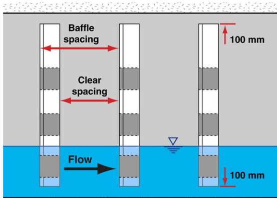
Full-height baffles
