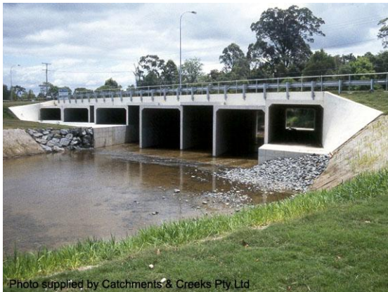
Multi-cell box culvert with wet & dry cells
