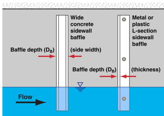
Baffle depth
