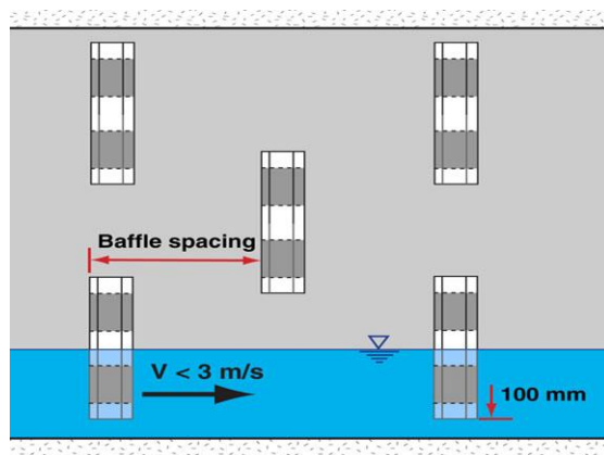
Tall culvert
