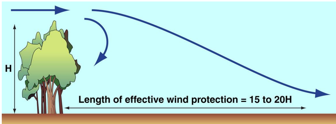
Figure F1 – Region of protection of soil from wind erosion downwind of a windbreak
