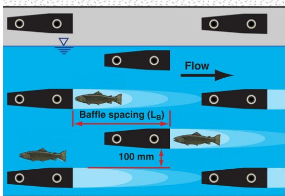
Sidewall roughness units
