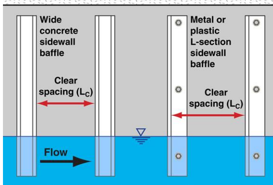
Baffle clear spacing
