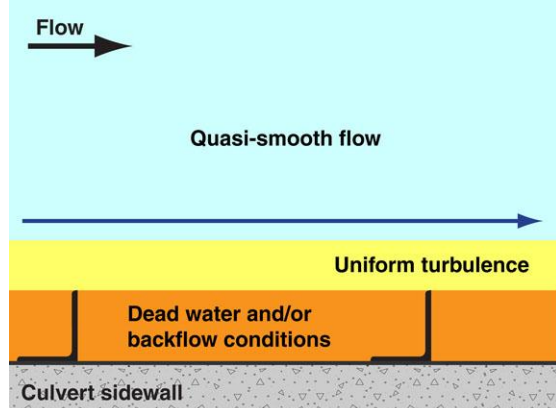
Quasi-smooth flow for L/k = 3.47
