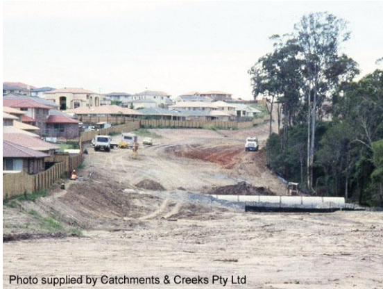
Early installation of stormwater pipe
