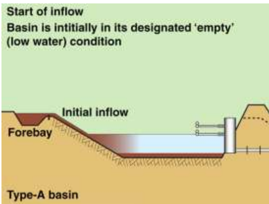
Initial filling of a Type A sediment basin
