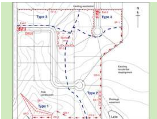
Site controls based on erosion risk
