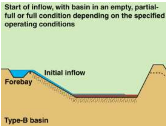
Initial filling of a Type B sediment basin
