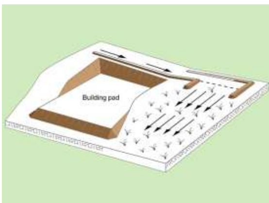
Use of a level spreader on a building site
