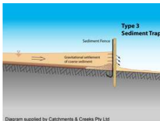
Type 3 sediment trap
