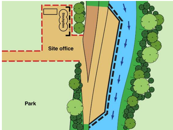
Conceptual ESCP for instream works
