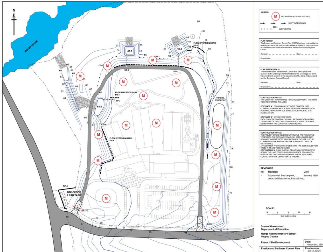
Figure 20 – Temporary erosion control measures on the Hodge Road school site
