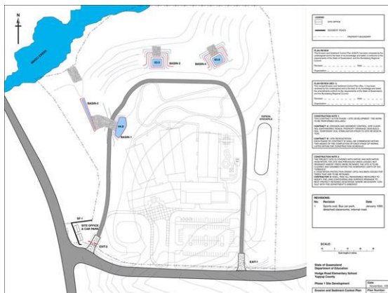
Placement of sediment basins
