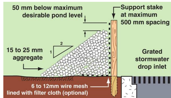
Construction detail
