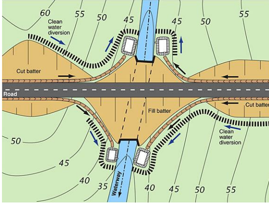
Culvert construction
