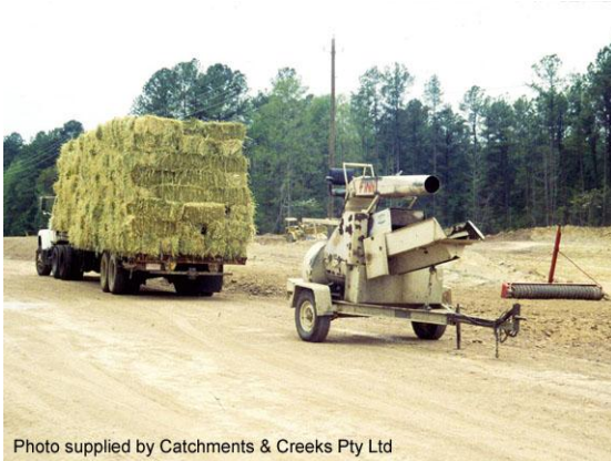
Straw blower
