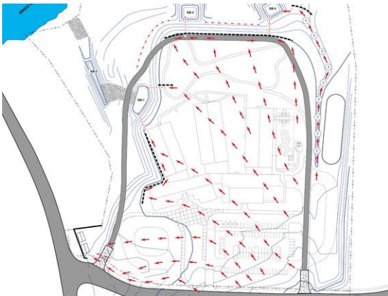
Post-earthworks drainage plan
