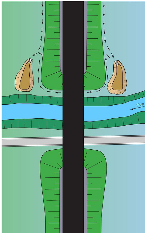
Final road layout with retained basins
