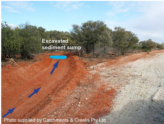
Excavated sediment trap/sump
