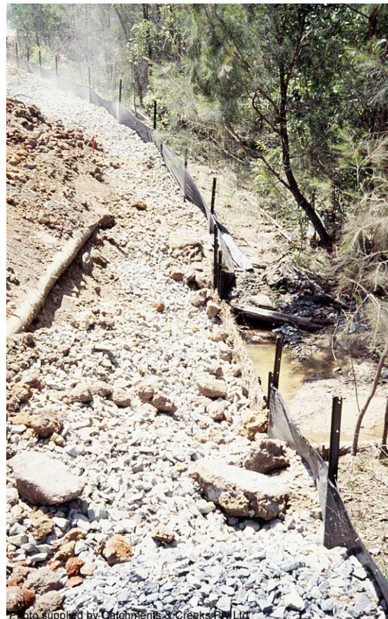
Spill-through weir & aggregate filter
