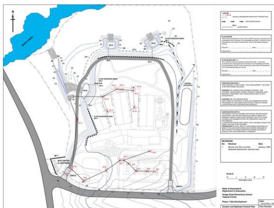
Placement of stormwater inlet traps
