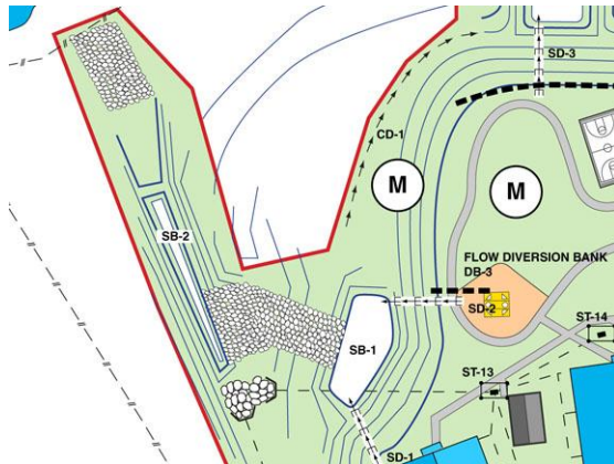
Sediment basins SB-1 and SB-2 in series
