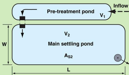
Type C basin with pre-treatment pond
