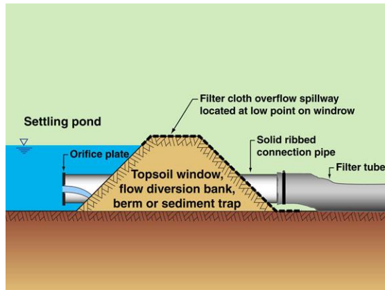
Topsoil windrow trap with filter tube
