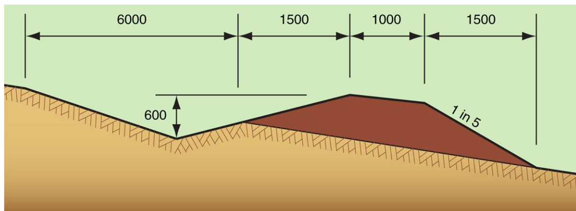
Wide, low-gradient, cross drainage berm (for higher speed tracks)
