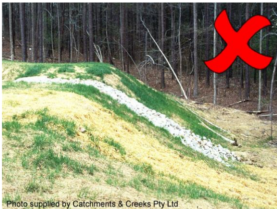
Insufficient scour protection at outlet
