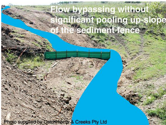
Sediment fence fails to capture sediment
