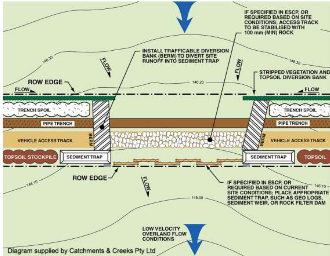
Example crossing of a medium to steep gradient drainage line
