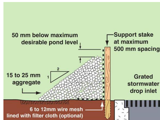
Construction detail
