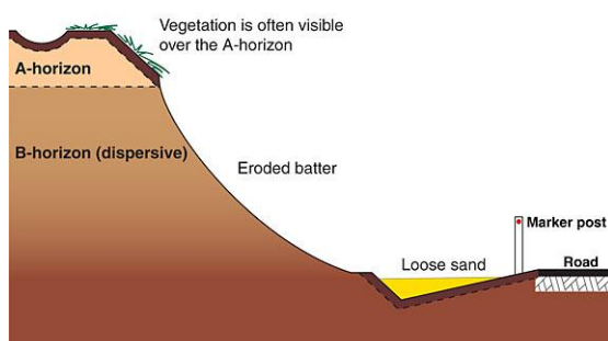
Eroded road batter
