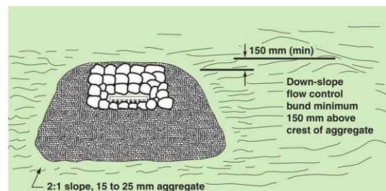
Flow diversion bank adjacent to drop inlet
