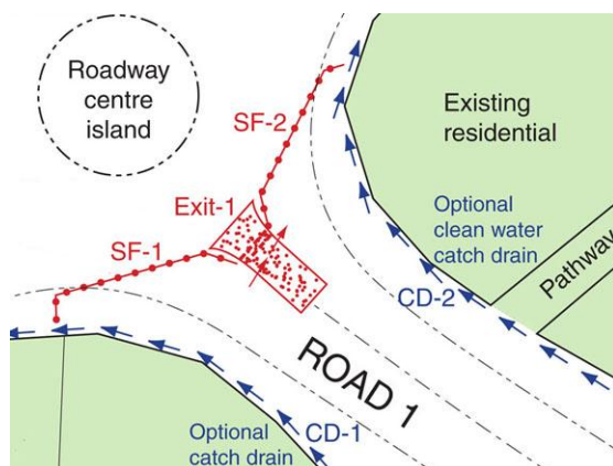
Progressive ESCP
