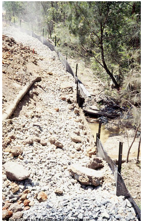
Spill-through weir & aggregate filter
