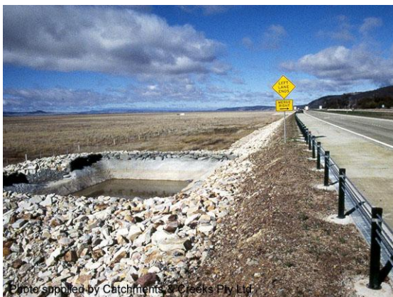
Roadside pollution containment pond
