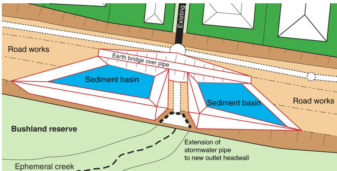
Figure 3 – Details of construction works ESCP at the pipe extension
