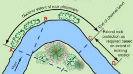
Placement of rock on channel bends
