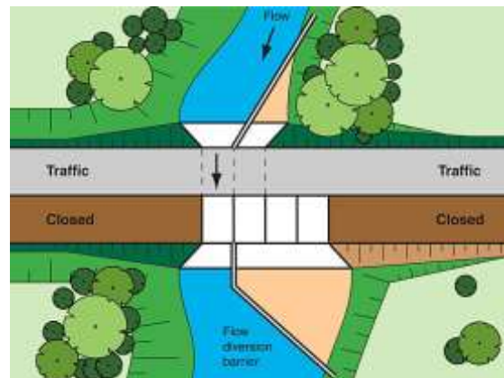
Case Study 4: Stage 2
