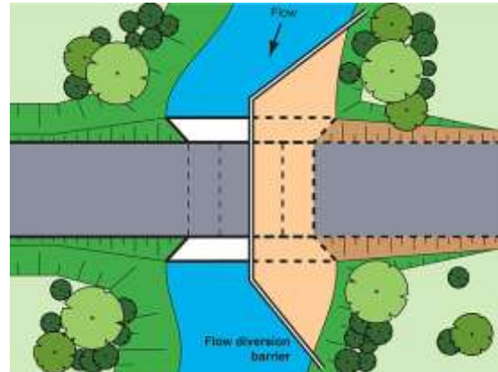
Case Study 3: Stage 2 of construction
